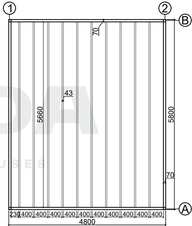
Base plan
