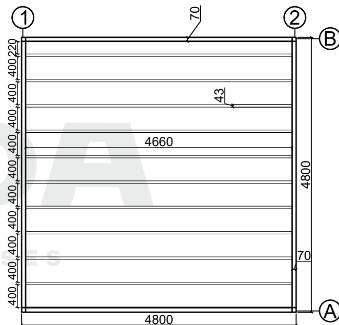
Base plan
