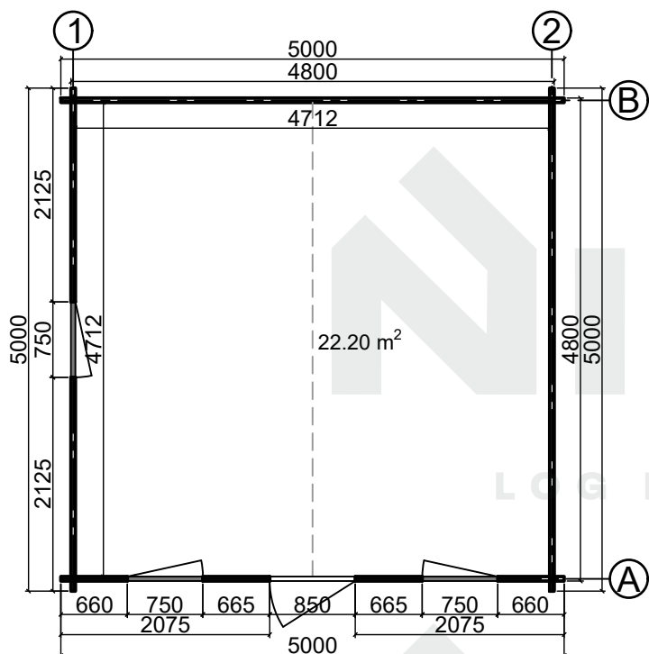
Floor plan
