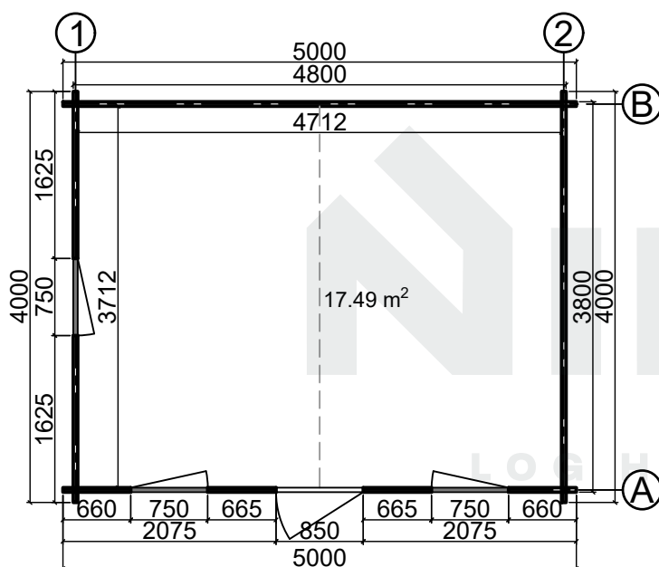
Floor plan
