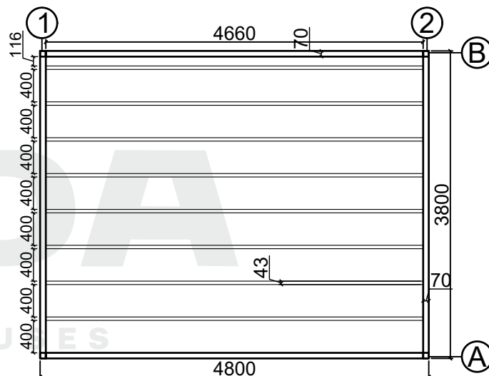
Base plan
