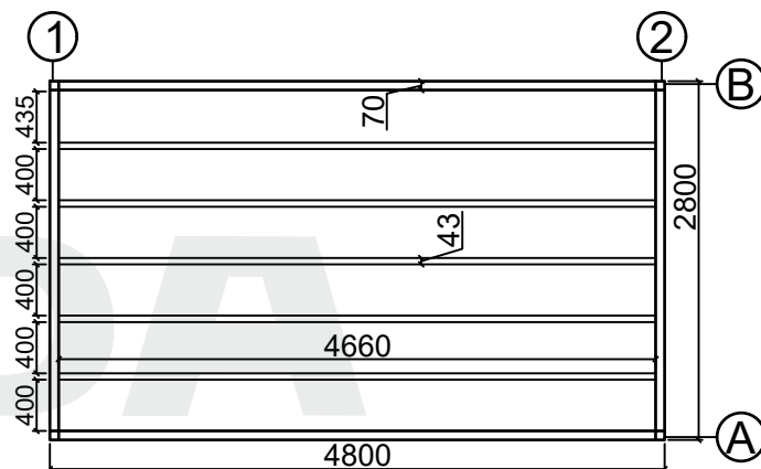
Base plan
