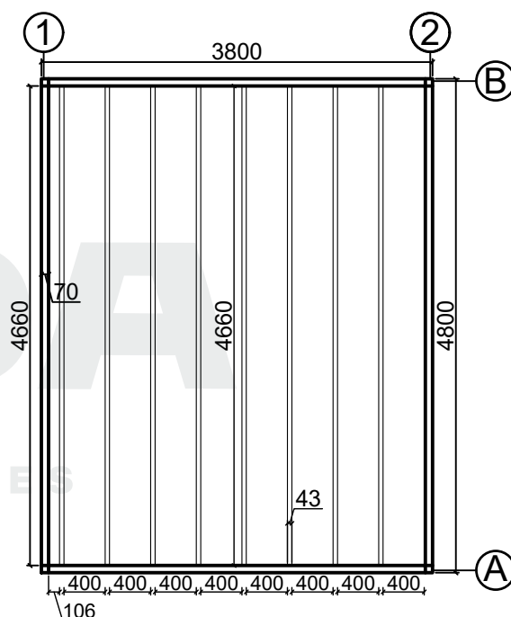
Base plan
