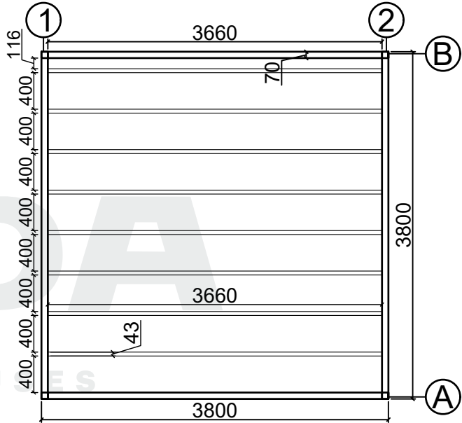
Base plan
