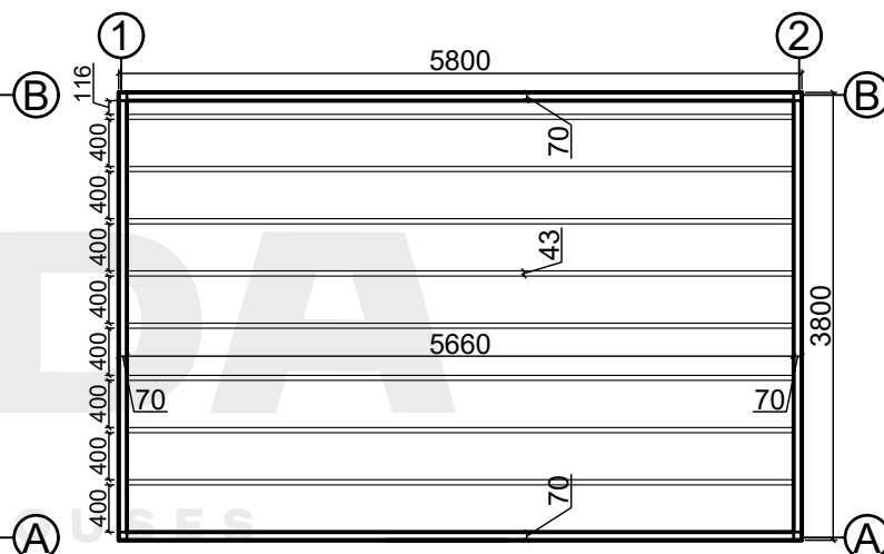
Base plan
