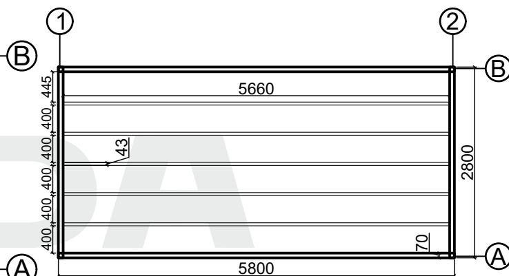
Base plan
