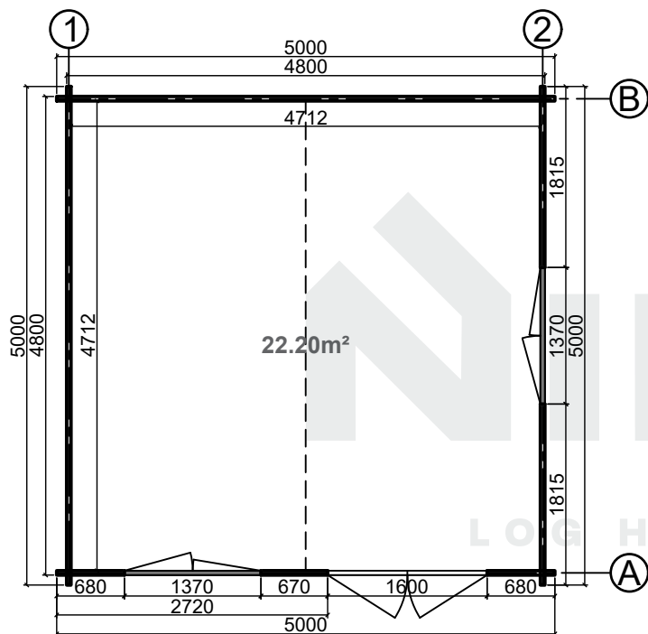
Floor plan
