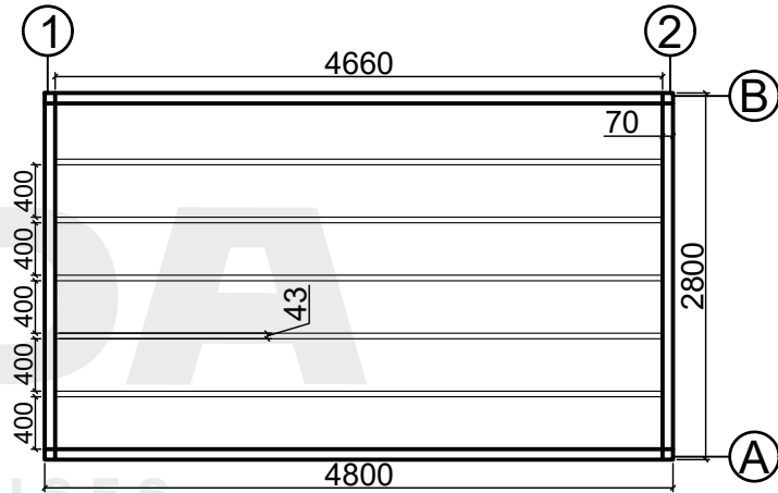
Base plan
