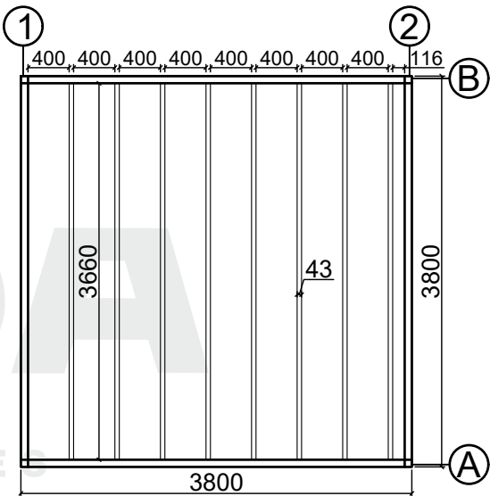
Base plan
