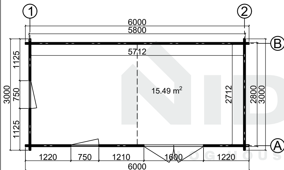
Floor plan
