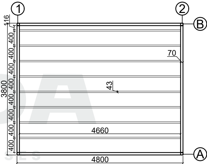
Base plan
