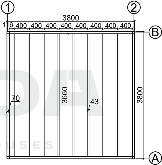
Base plan
