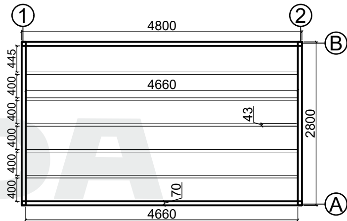
Base plan
