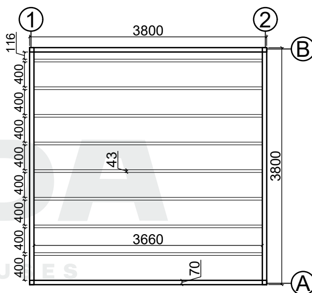
Base plan
